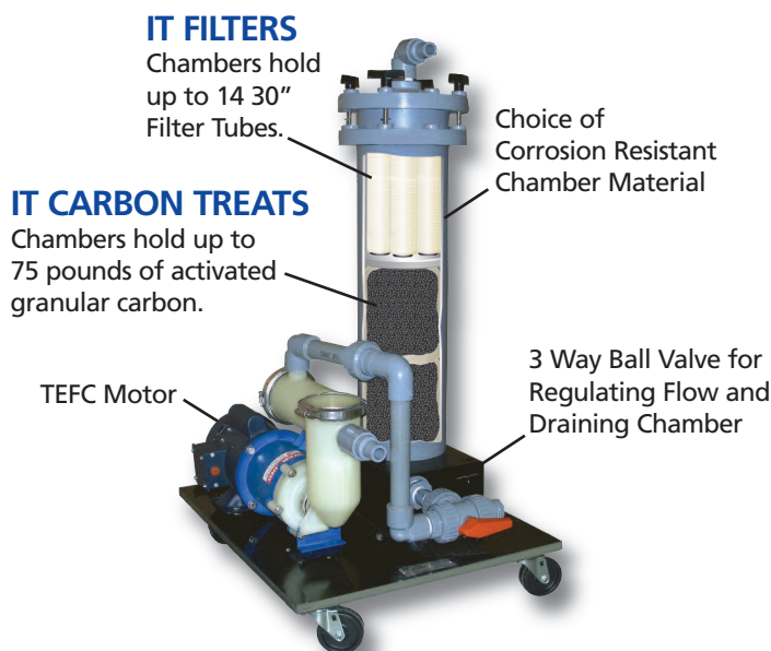
The Sethco In-Filtrator is designed for fast and easy tube and carbon replacement. The entire chamber can be disassembled and reassembled in minutes.
